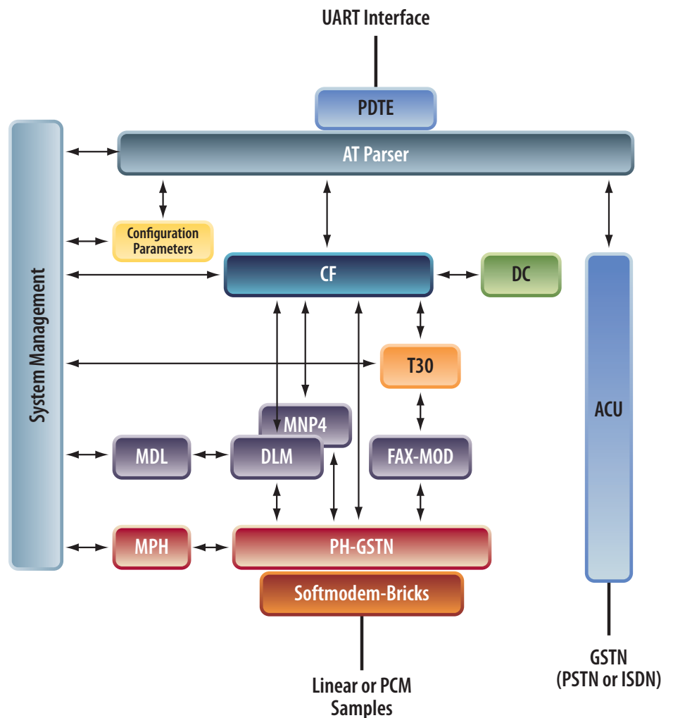
CLIENT MODEM SOFTWARE ARCHITECTURE
